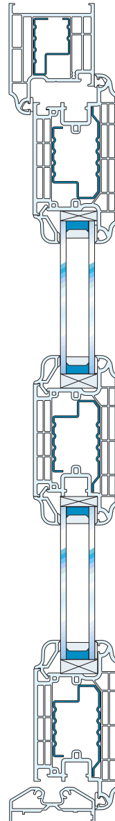
Outward opening. Internally beaded. Using Aluminium low threshold.
