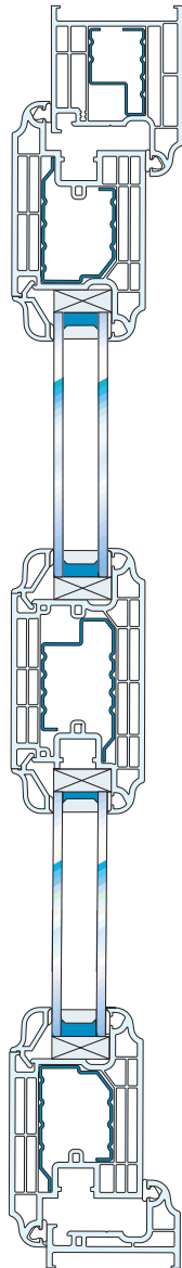
Inward opening. Internally beaded. Using PVC low threshold.
