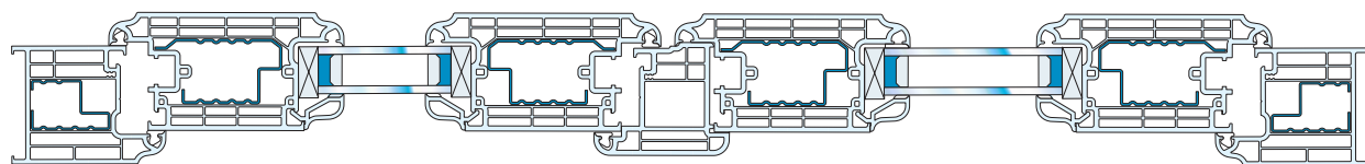
Outward opening. Internally beaded.
